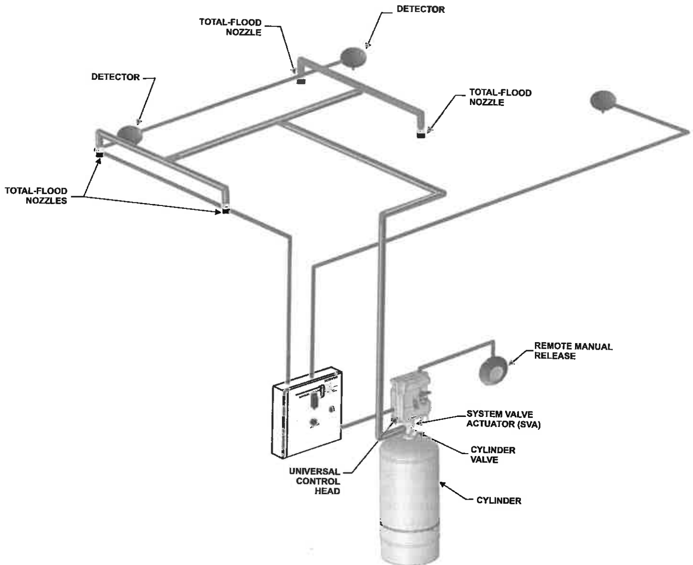
Figure 1-1. Typical Badger Industry Guard Dry Chemical Fire Suppression System.
